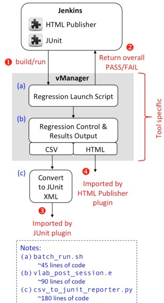
Figure 2: Overview of Jenkins/vManager Integration
